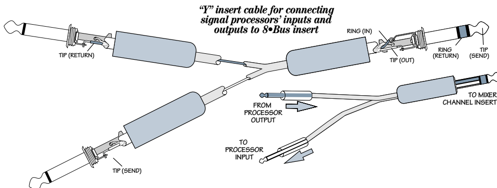
Figure 4: Common Connectors
